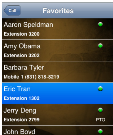
Figure 15. Favorites view
